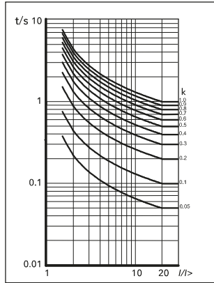
NORMAL INVERSE 1.3/10
