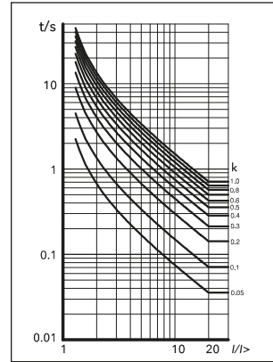
VERY INVERSE
