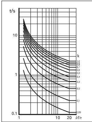
NORMAL INVERSE 3/10
