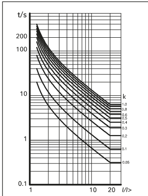
LONG-TIME INVERSE
