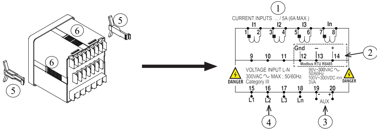
Figure 1: Parts of power meter
