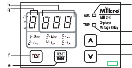
Figure 1: Front panel overview
